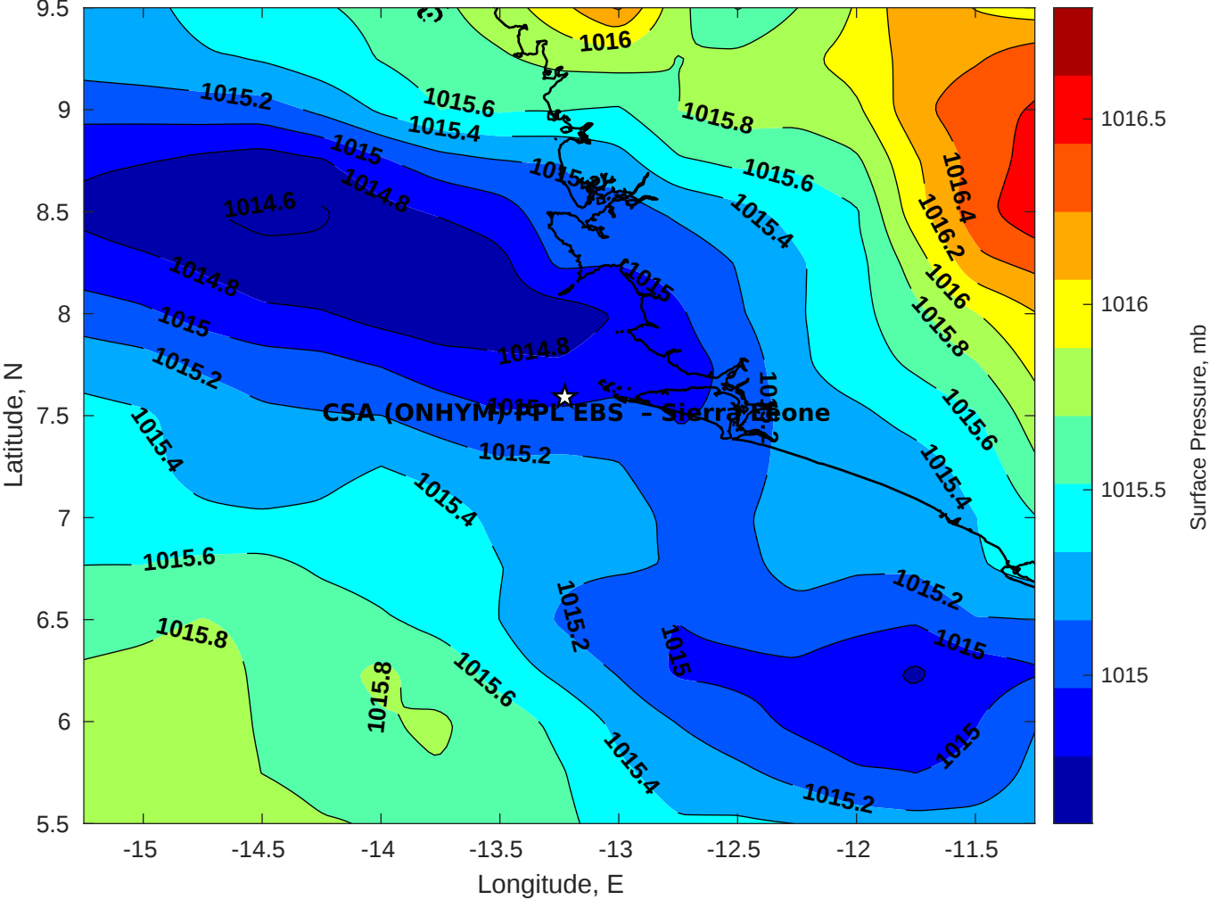
Surface Pressure (mb) for CSA (ONHYM) PPL EBS - Sierra Leone at 08-Feb-2026 00:00:00
