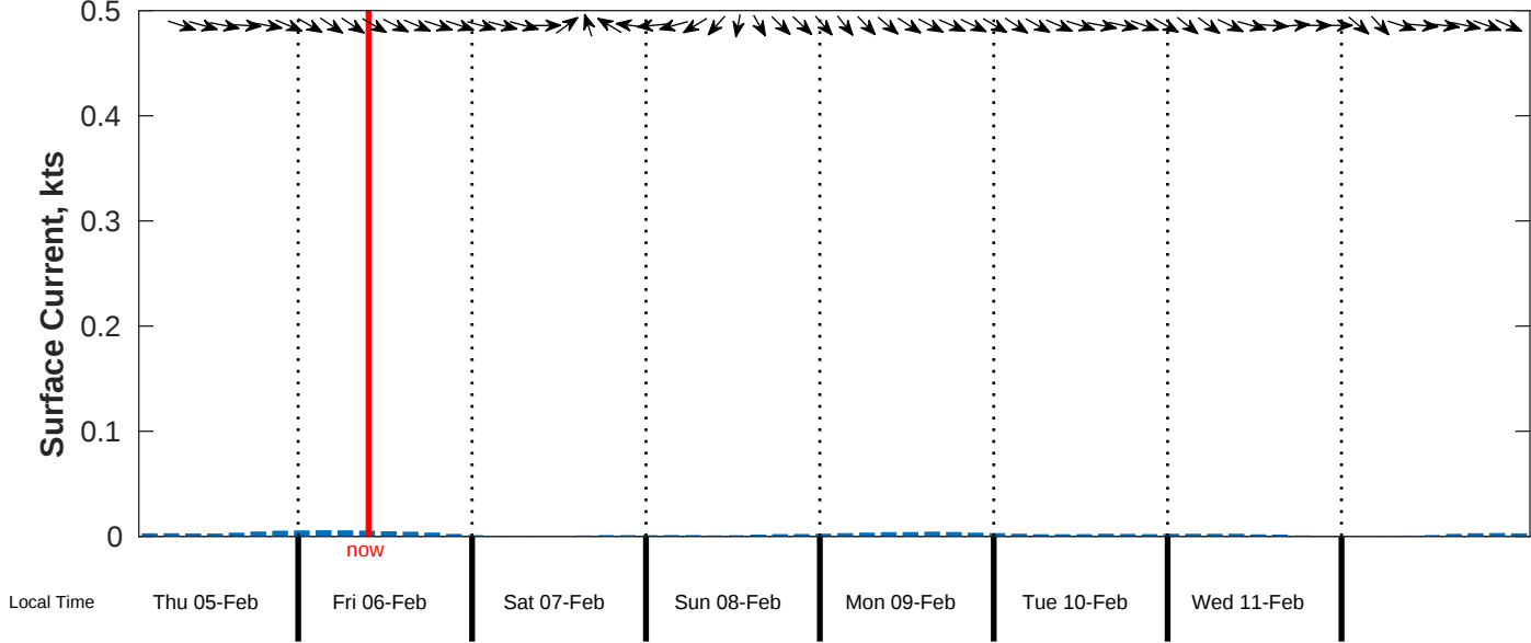
Surface Current Forecast for CSA (ONHYM) PPL EBS - Sierra Leone from 05-Feb-2026 00:00:00 to 13-Feb-2026 00:00:00
