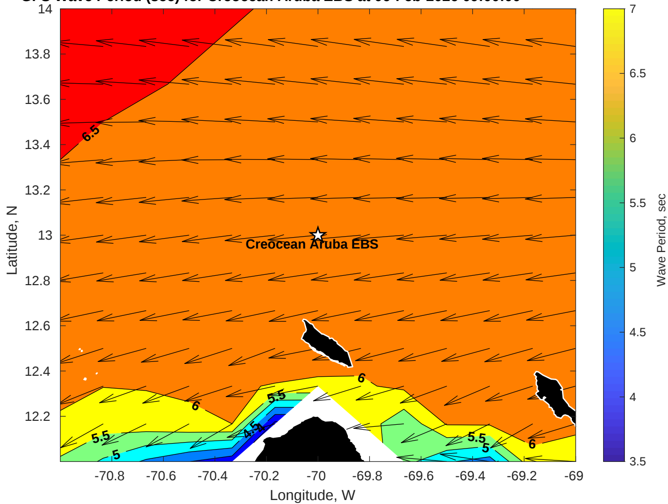
GFS Wave Period (sec) for Creoccean Aruba EBS at 06-Feb-2026 09:00:00
