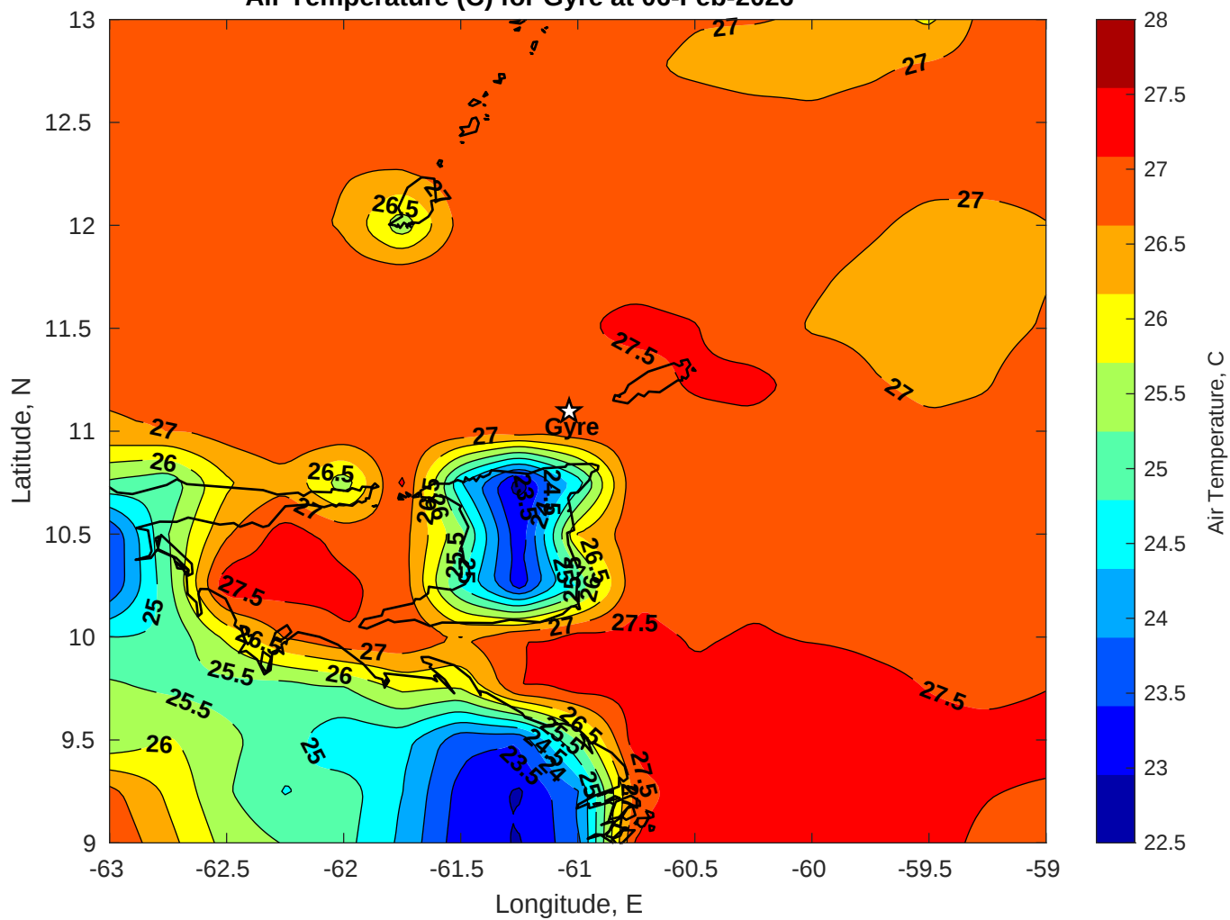
Air Temperature (C) for Gyre at 06-Feb-2026
