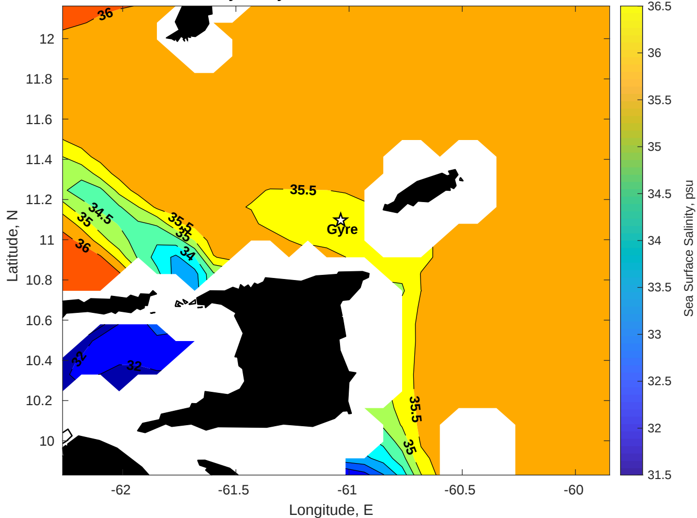
Surface Salinity for Gyre at 05-Feb-2026 00:00:00
