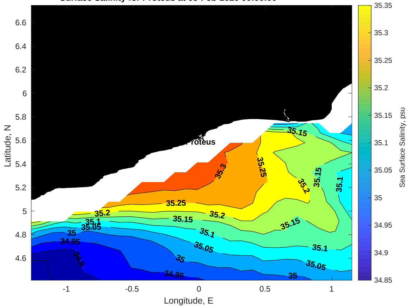
Surface Salinity for Proteus at 05-Feb-2026 00:00:00
