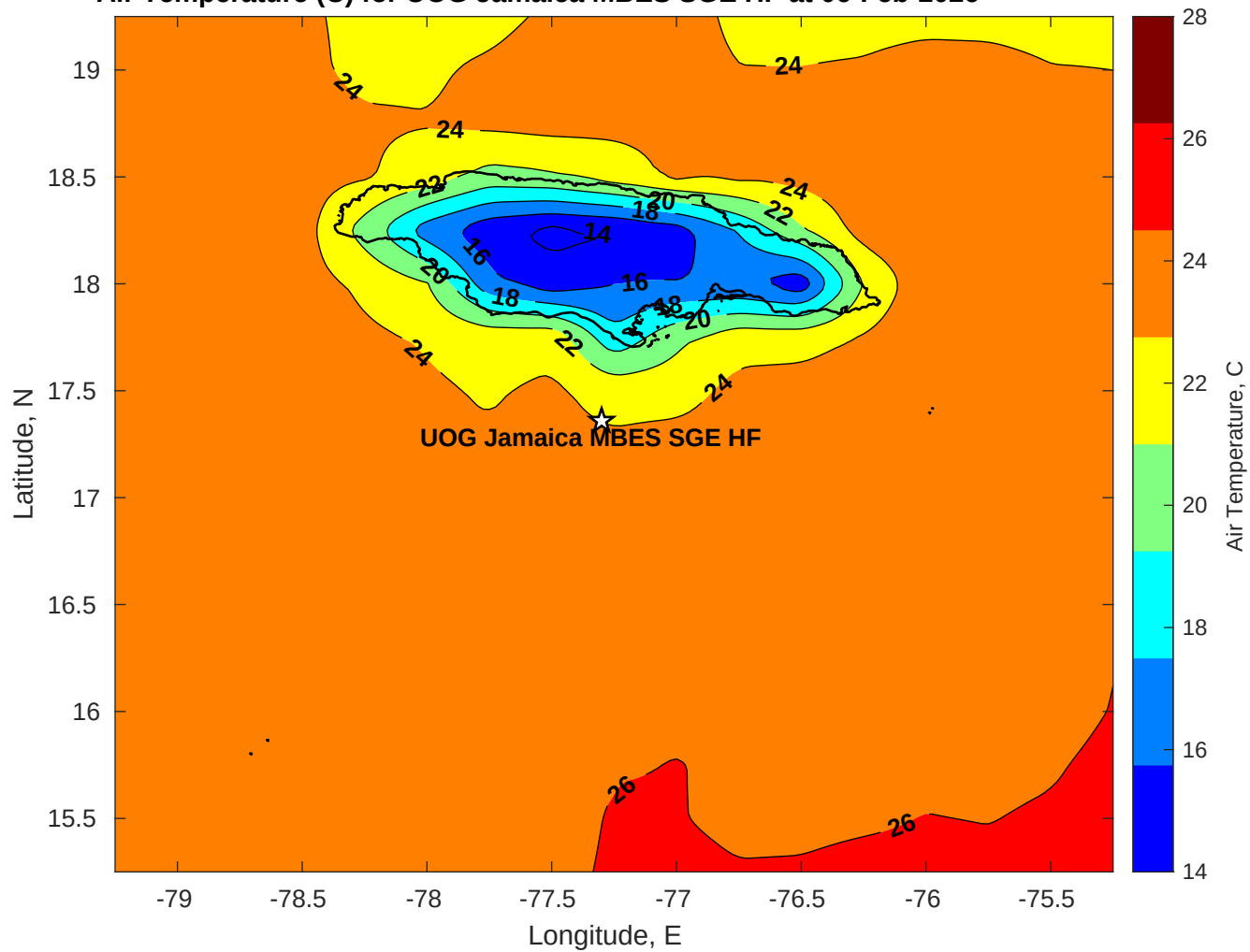
Air Temperature (C) for UOG Jamaica MBES SGE HF at 06-Feb-2026
