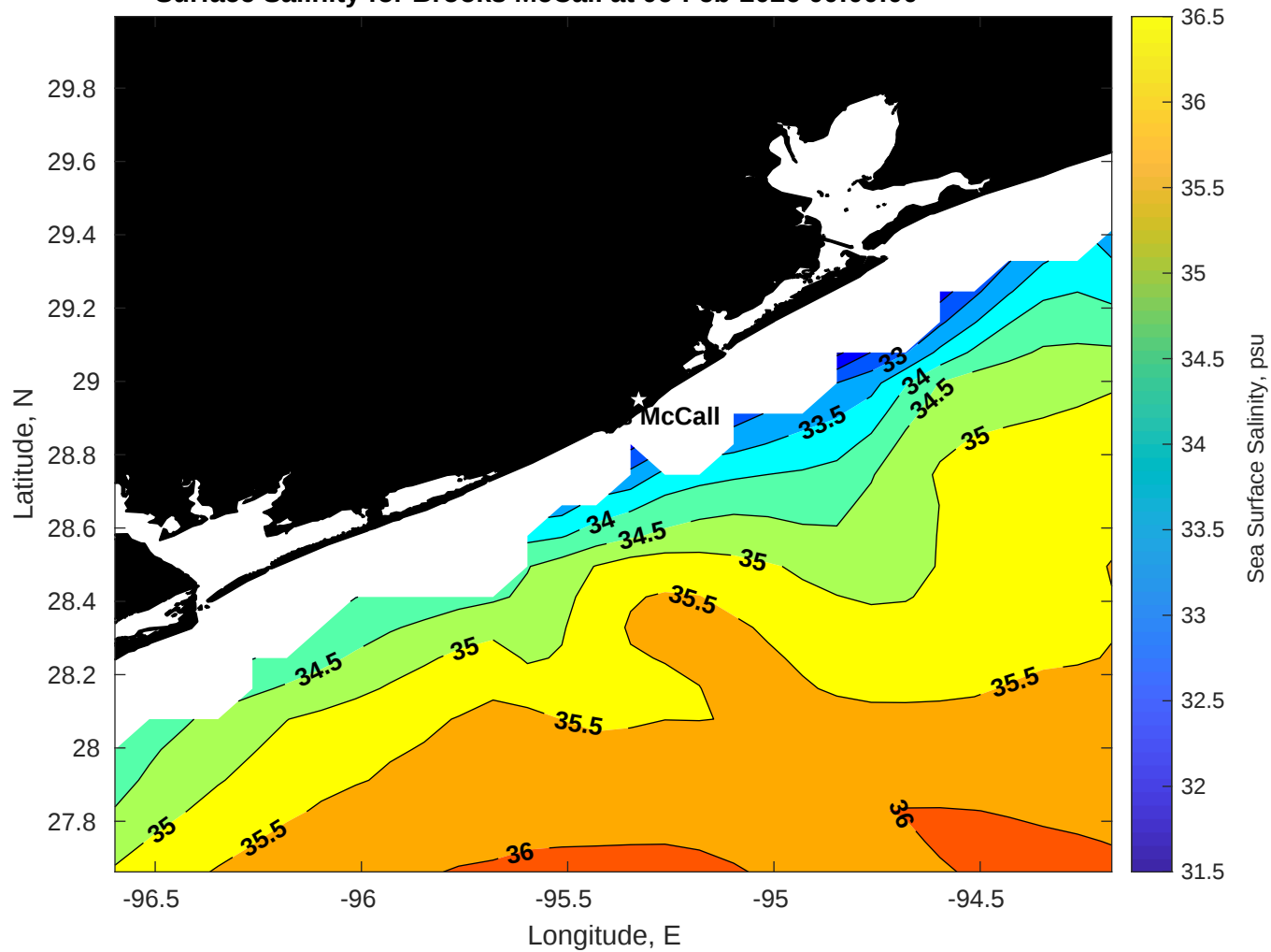
Surface Salinity for Brooks McCall at 06-Feb-2026 00:00:00
