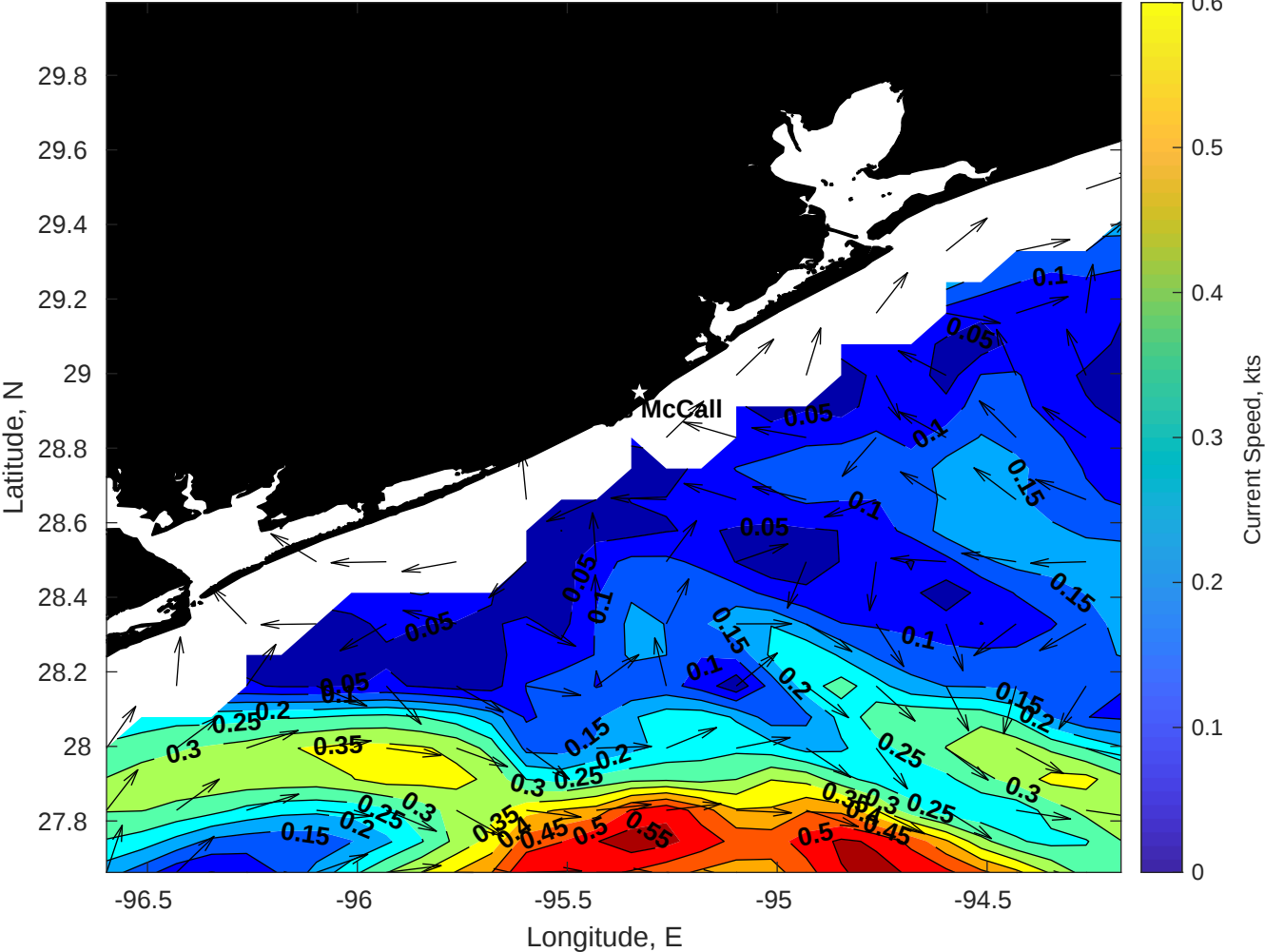
Surface Currents for Brooks McCall at 06-Feb-2026 00:00:00
