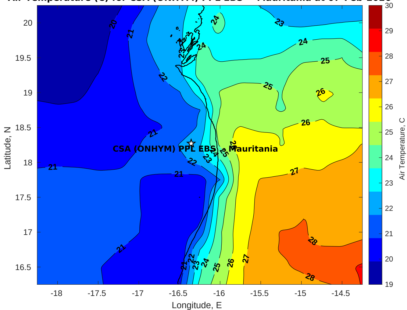
Air Temperature (C) for CSA (ONHYM) PPL EBS - Mauritania at 07-Feb-2026
