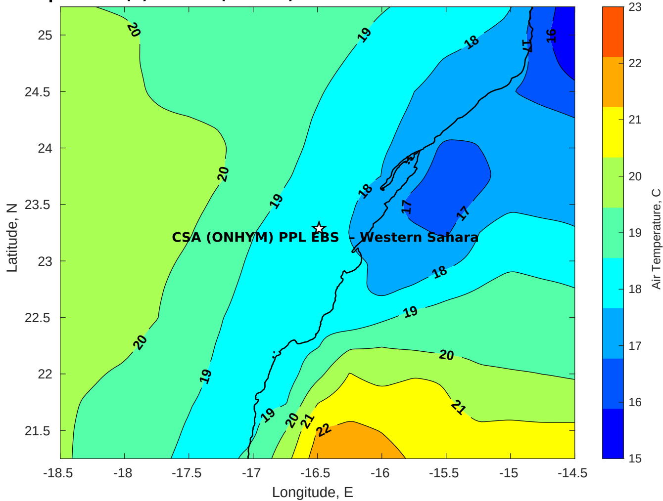
Air Temperature (C) for CSA (ONHYM) PPL EBS - Western Sahara at 07-Feb-2026
