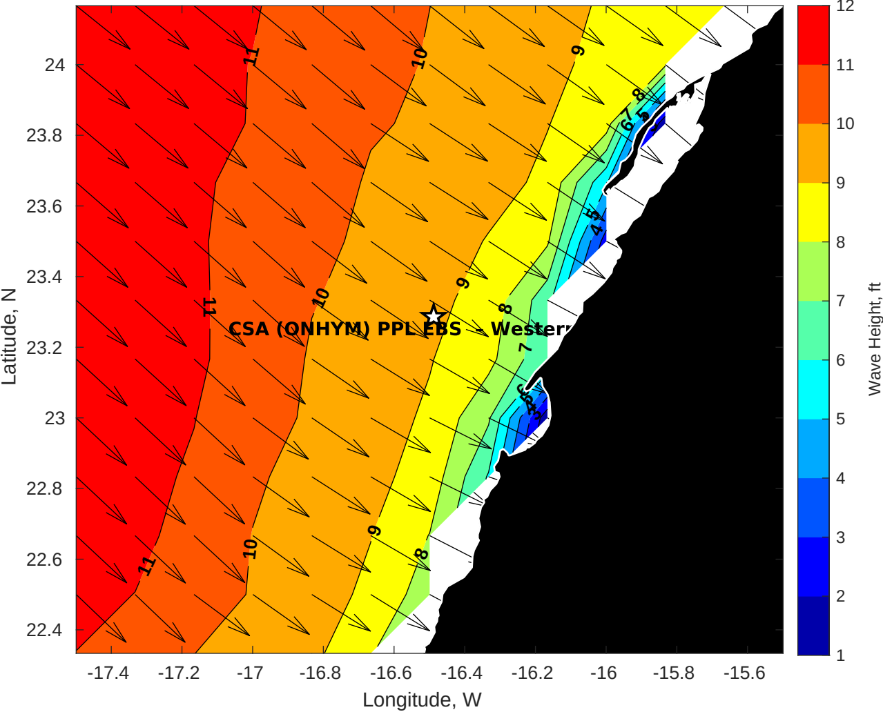
GFS Wave Height (ft) for CSA (ONHYM) PPL EBS - Western Sahara at 07-Feb-2026 09:00:00
