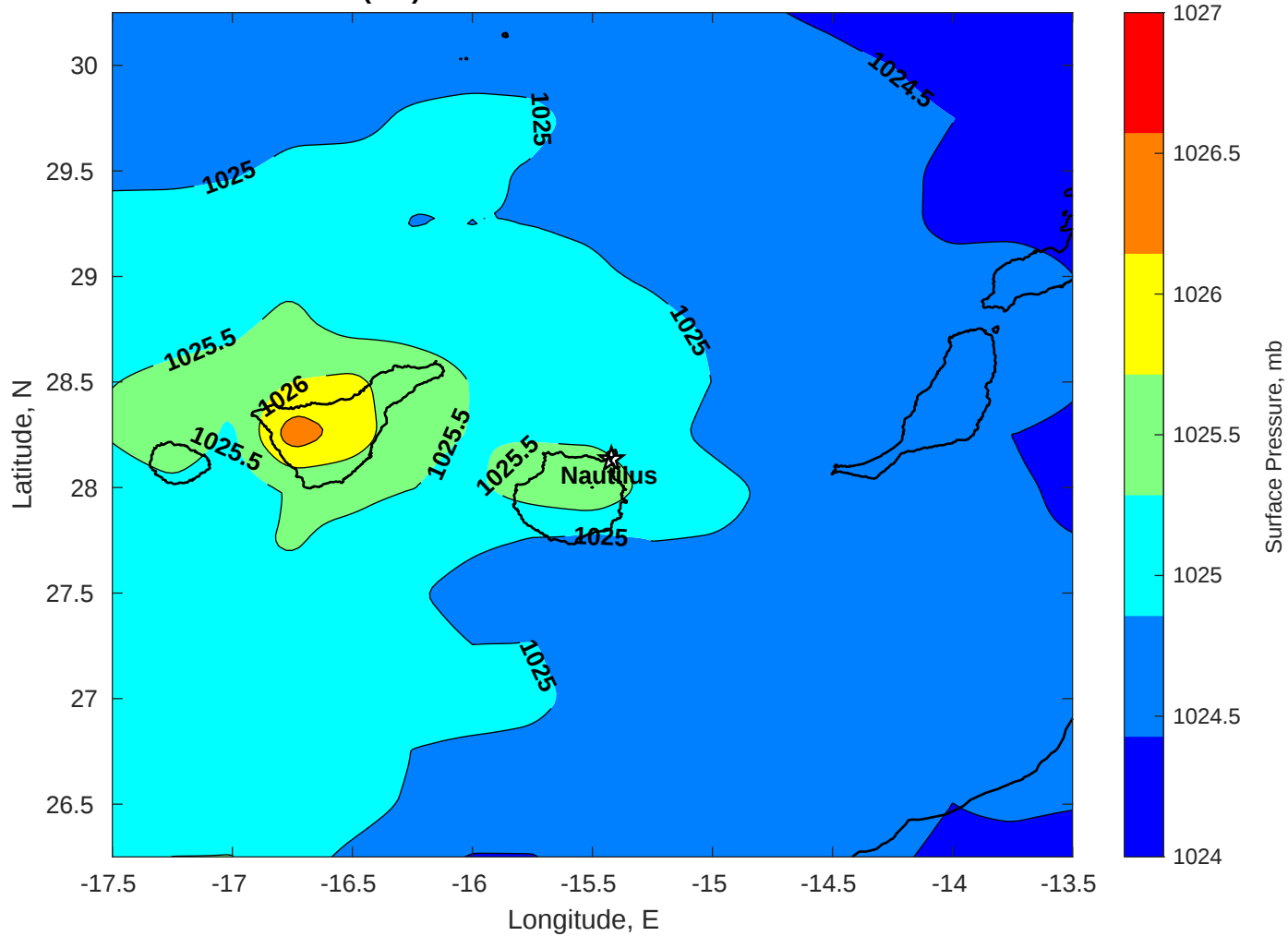
Surface Pressure (mb) for Nautilus at 07-Feb-2026 00:00:00
