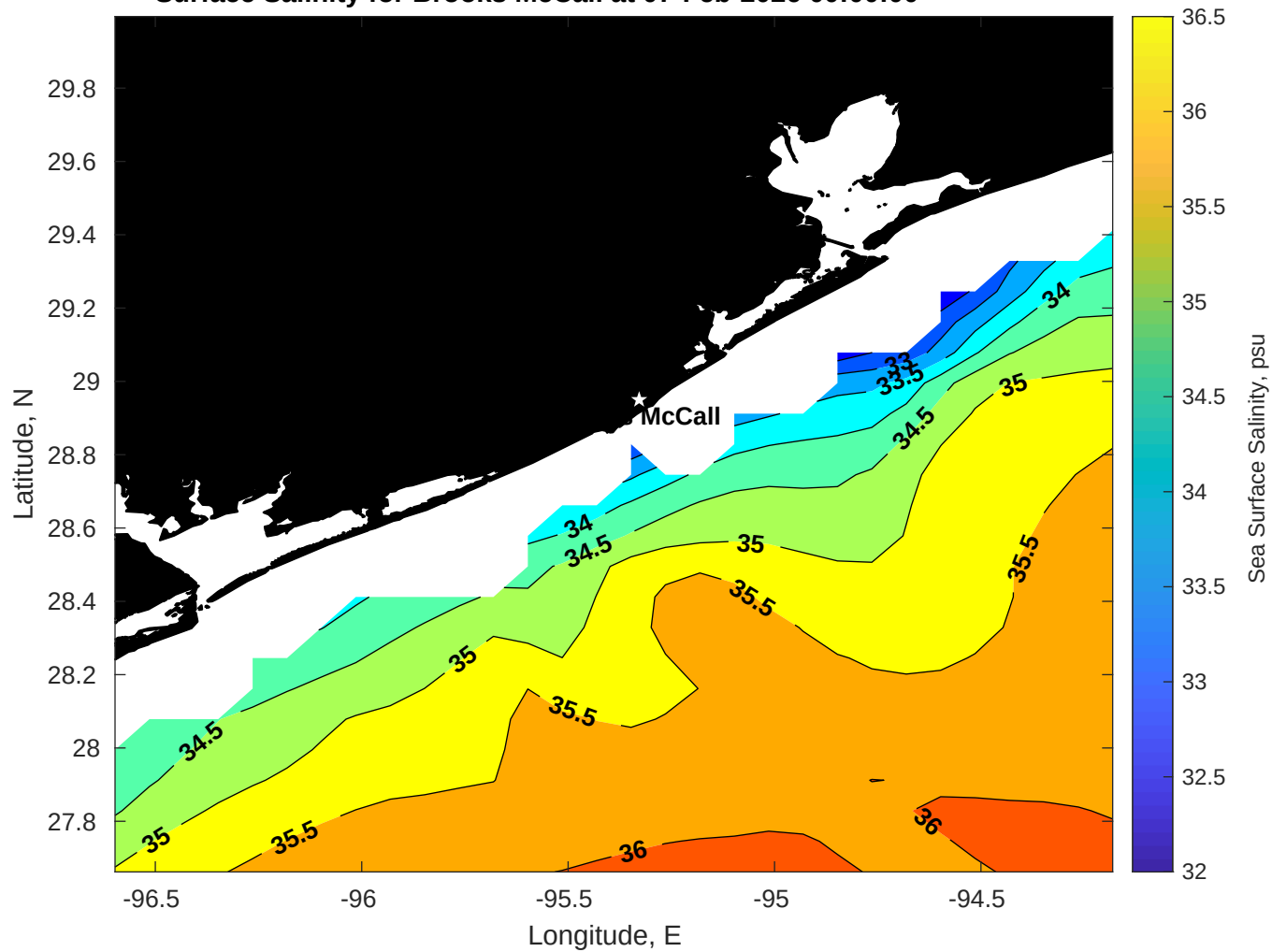
Surface Salinity for Brooks McCall at 07-Feb-2026 00:00:00
