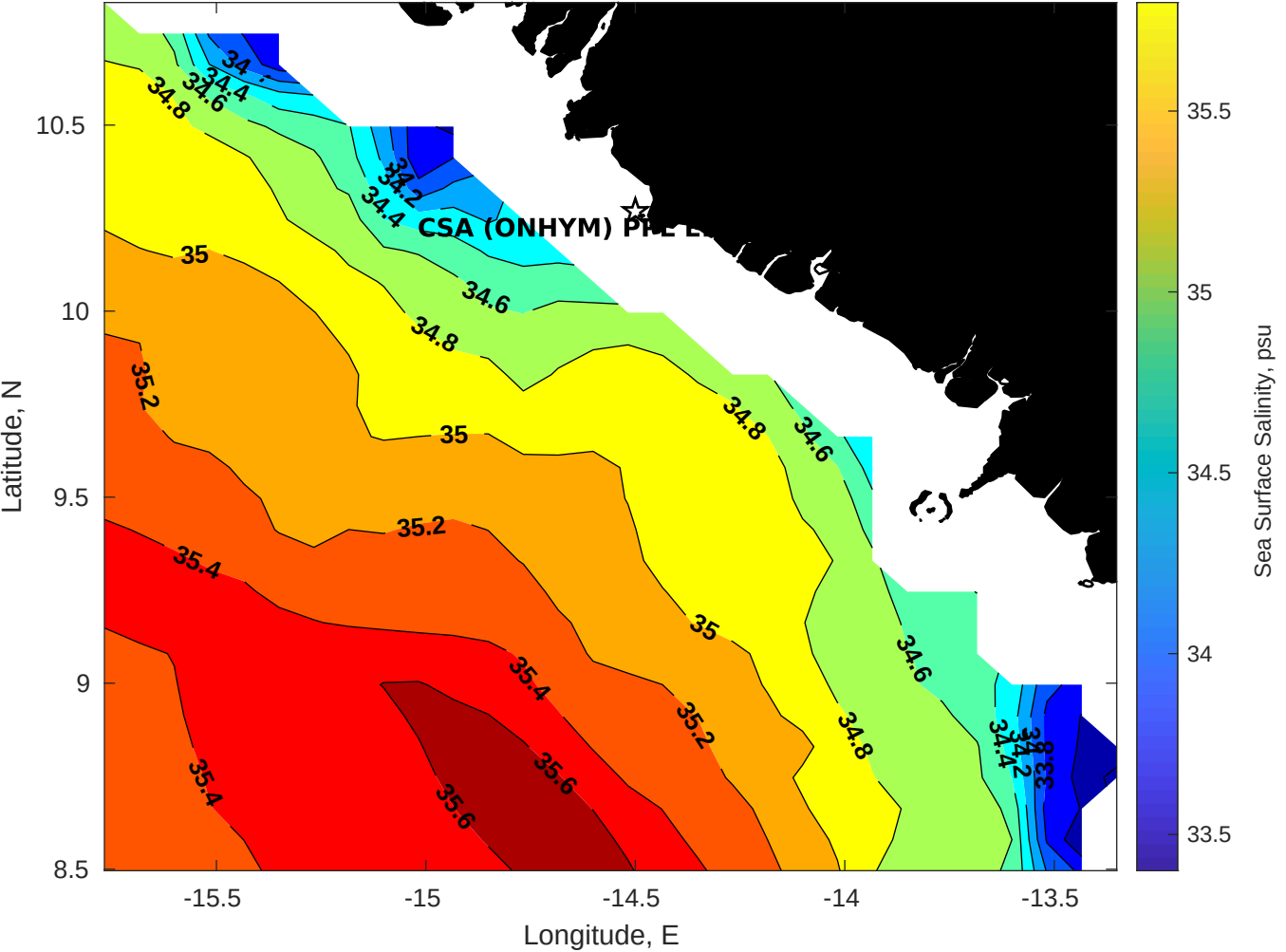
Surface Salinity for CSA (ONHYM) PPL EBS - Guinea at 07-Feb-2026 00:00:00
