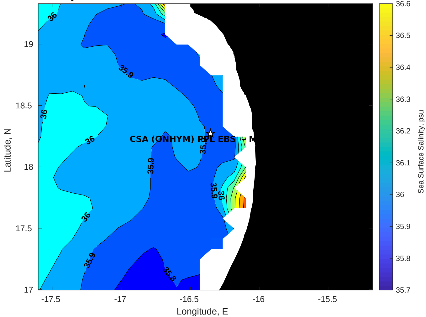
Surface Salinity for CSA (ONHYM) PPL EBS - Mauritania at 07-Feb-2026 00:00:00
