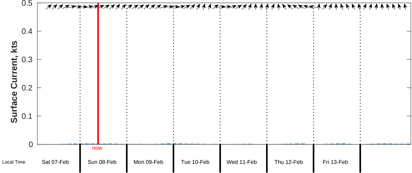
Surface Current Forecast for CSA (ONHYM) PPL EBS - Mauritania from 07-Feb-2026 00:00:00 to 15-Feb-2026 00:00:00
