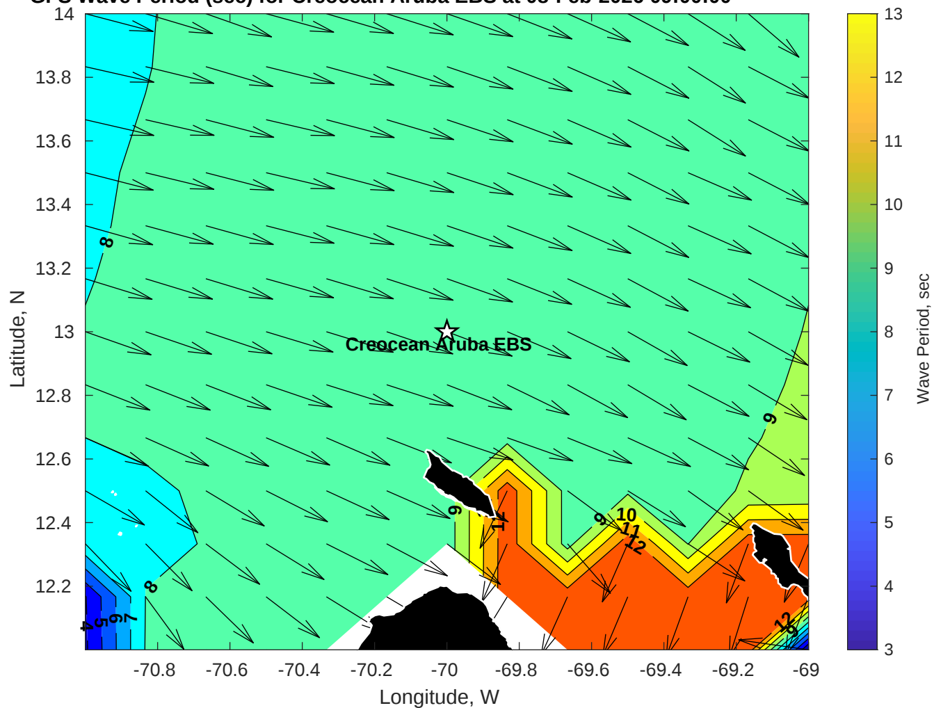
GFS Wave Period (sec) for Creoccean Aruba EBS at 08-Feb-2026 09:00:00
