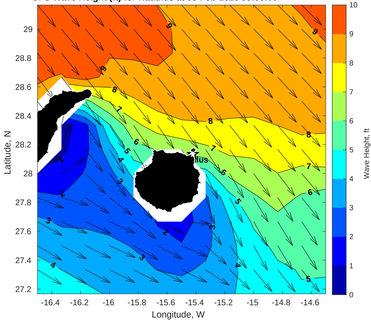
GFS Wave Height (ft) for Nautilus at 08-Feb-2026 09:00:00
