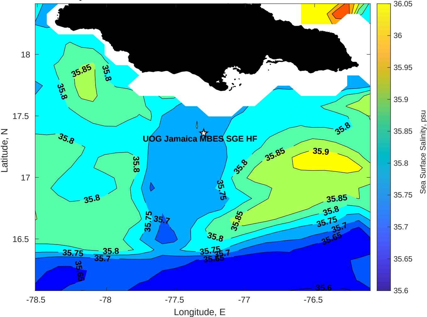
Surface Salinity for UOG Jamaica MBES SGE HF at 07-Feb-2026 00:00:00
