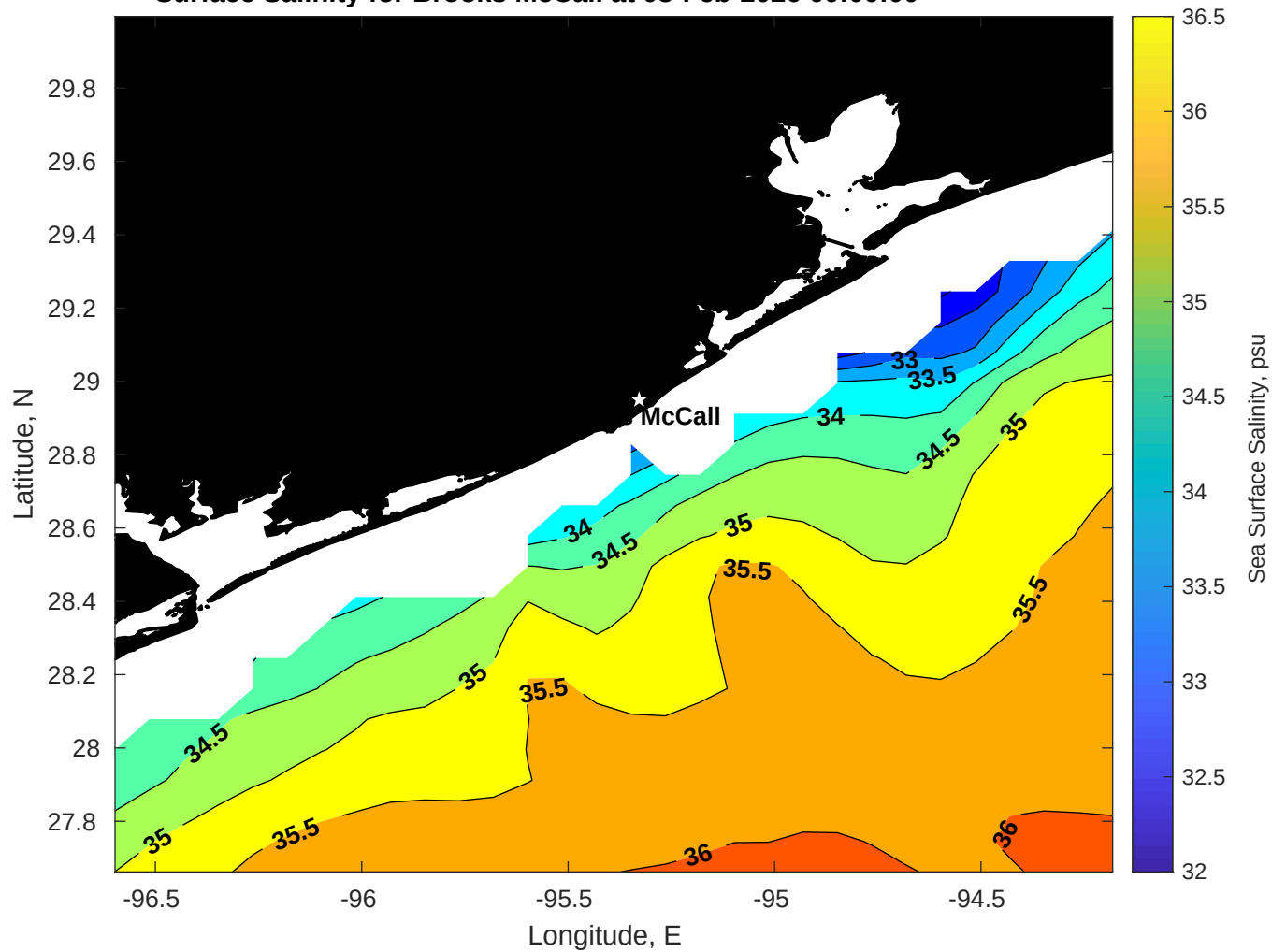
Surface Salinity for Brooks McCall at 08-Feb-2026 00:00:00
