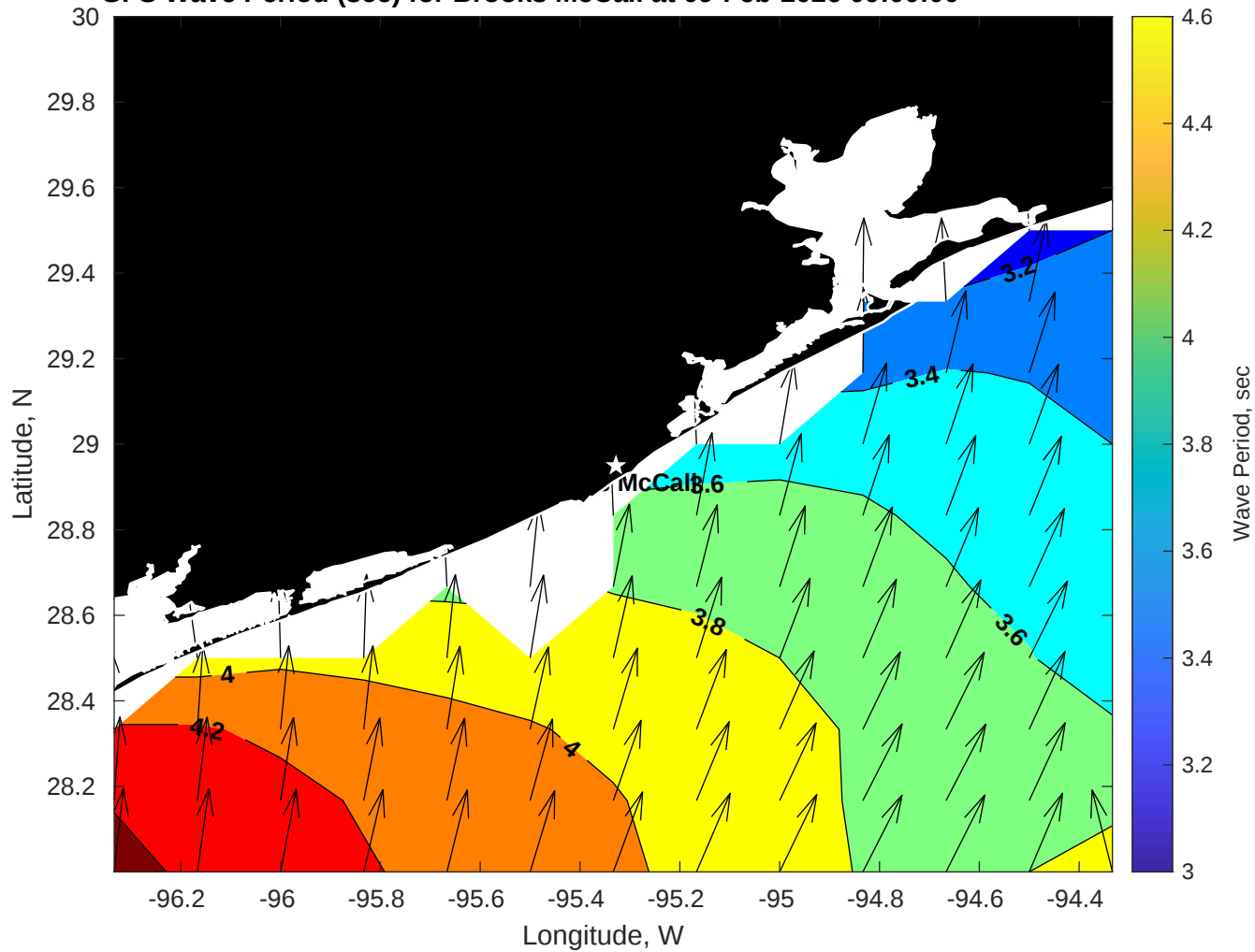
GFS Wave Period (sec) for Brooks McCall at 09-Feb-2026 09:00:00
