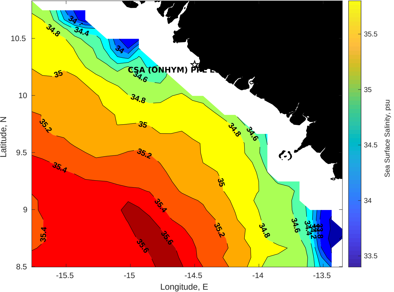
Surface Salinity for CSA (ONHYM) PPL EBS - Guinea at 08-Feb-2026 00:00:00
