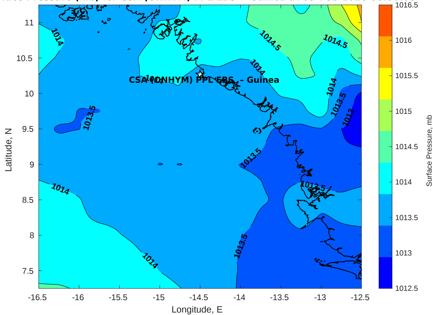
Surface Pressure (mb) for CSA (ONHYM) PPL EBS - Guinea at 09-Feb-2026 00:00:00
