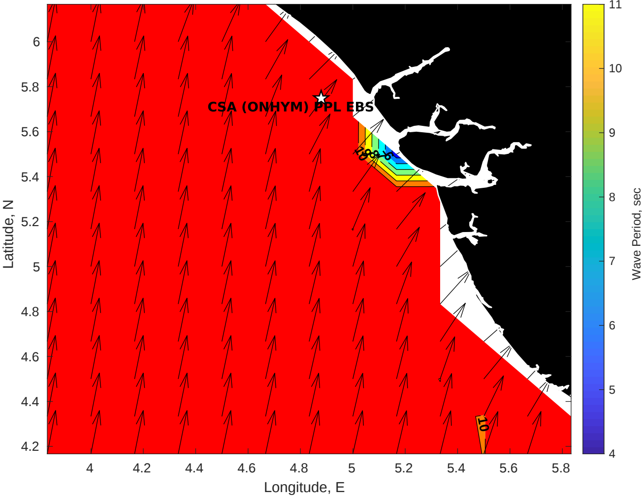
GFS Wave Period (sec) for CSA (ONHYM) PPL EBS - Nigeria at 09-Feb-2026 09:00:00
