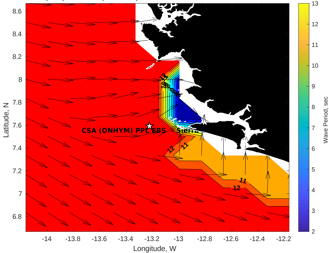
GFS Wave Period (sec) for CSA (ONHYM) PPL EBS - Sierra Leone at 09-Feb-2026 09:00:00
