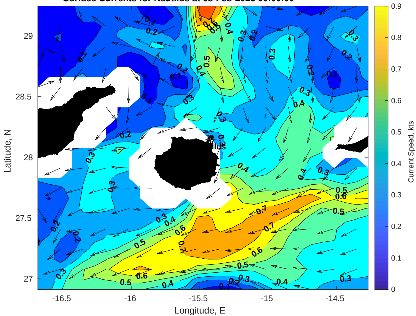
Surface Currents for Nautilus at 08-Feb-2026 00:00:00
