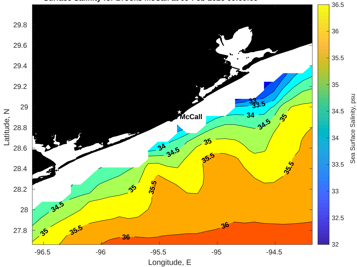
Surface Salinity for Brooks McCall at 09-Feb-2026 00:00:00
