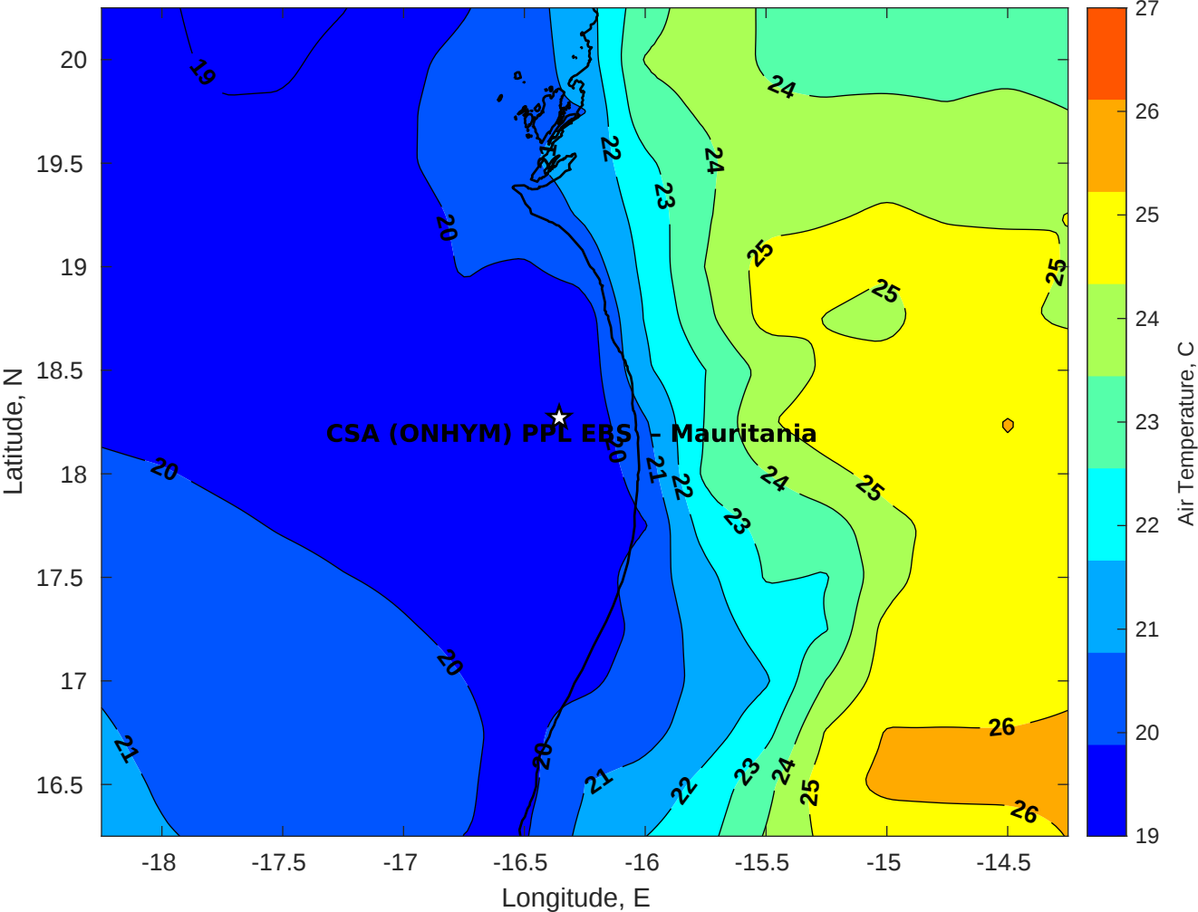
Air Temperature (C) for CSA (ONHYM) PPL EBS - Mauritania at 10-Feb-2026
