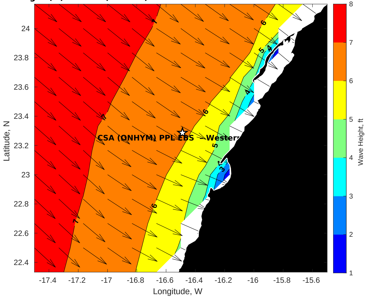
GFS Wave Height (ft) for CSA (ONHYM) PPL EBS - Western Sahara at 10-Feb-2026 09:00:00
