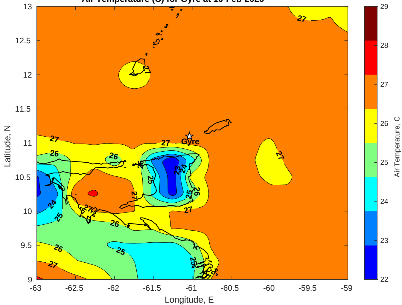
Air Temperature (C) for Gyre at 10-Feb-2026
