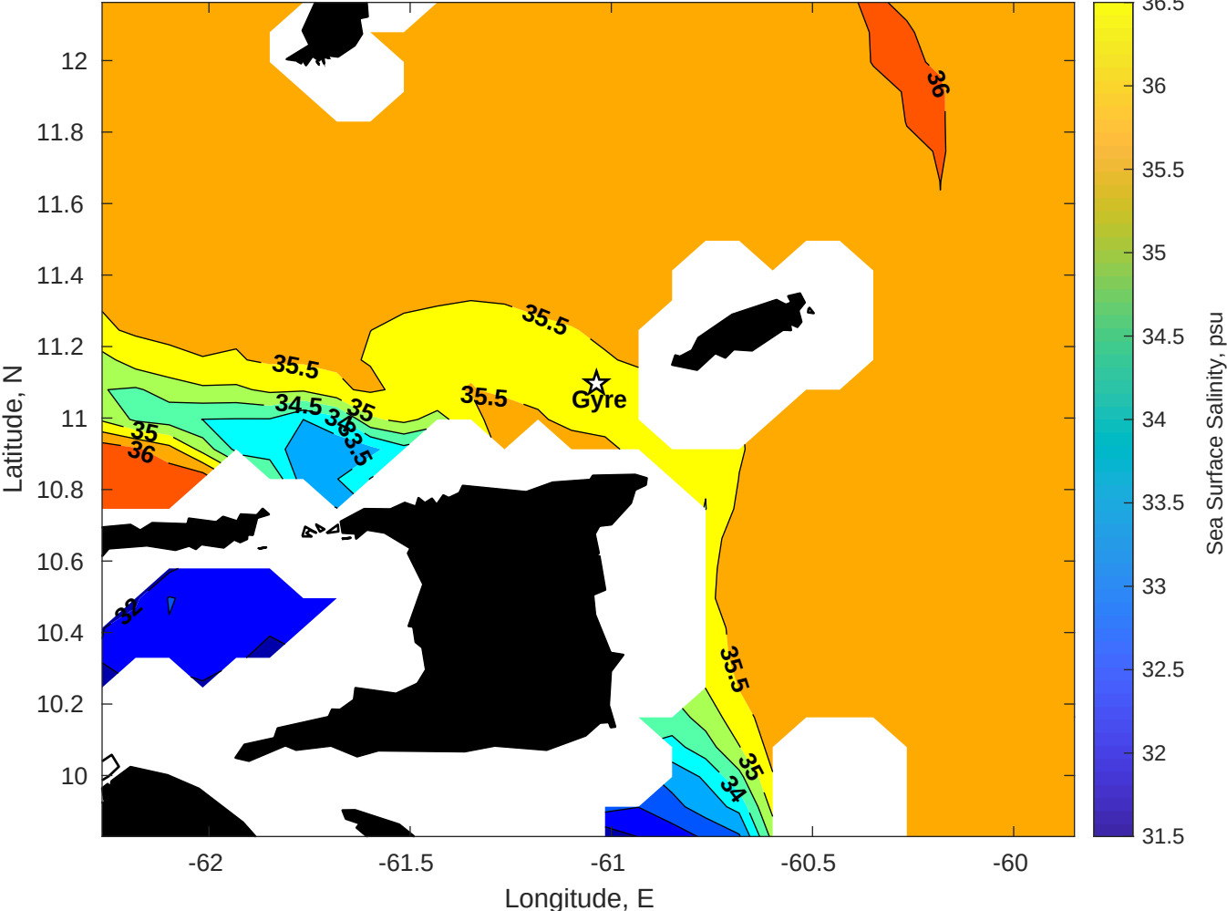
Surface Salinity for Gyre at 09-Feb-2026 00:00:00
