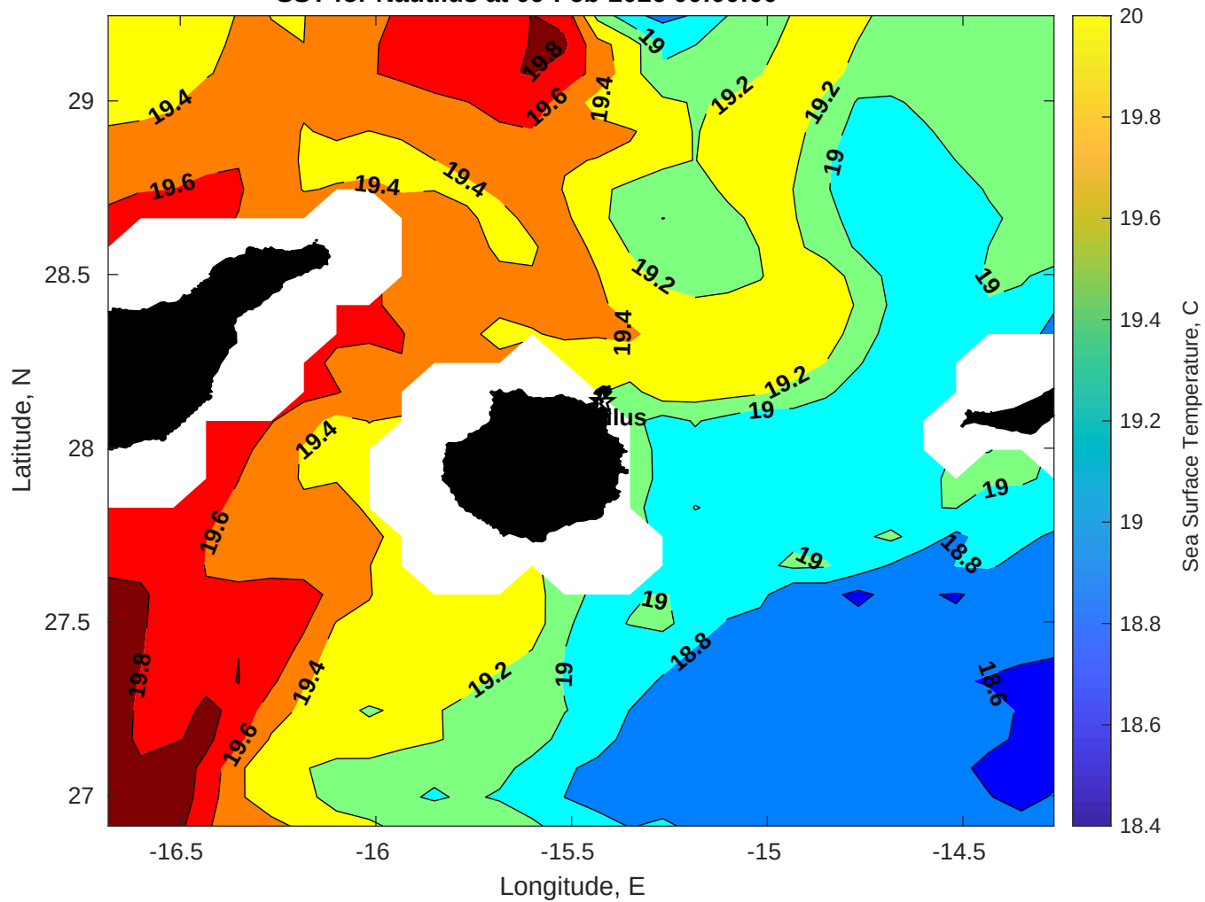
SST for Nautilus at 09-Feb-2026 00:00:00
