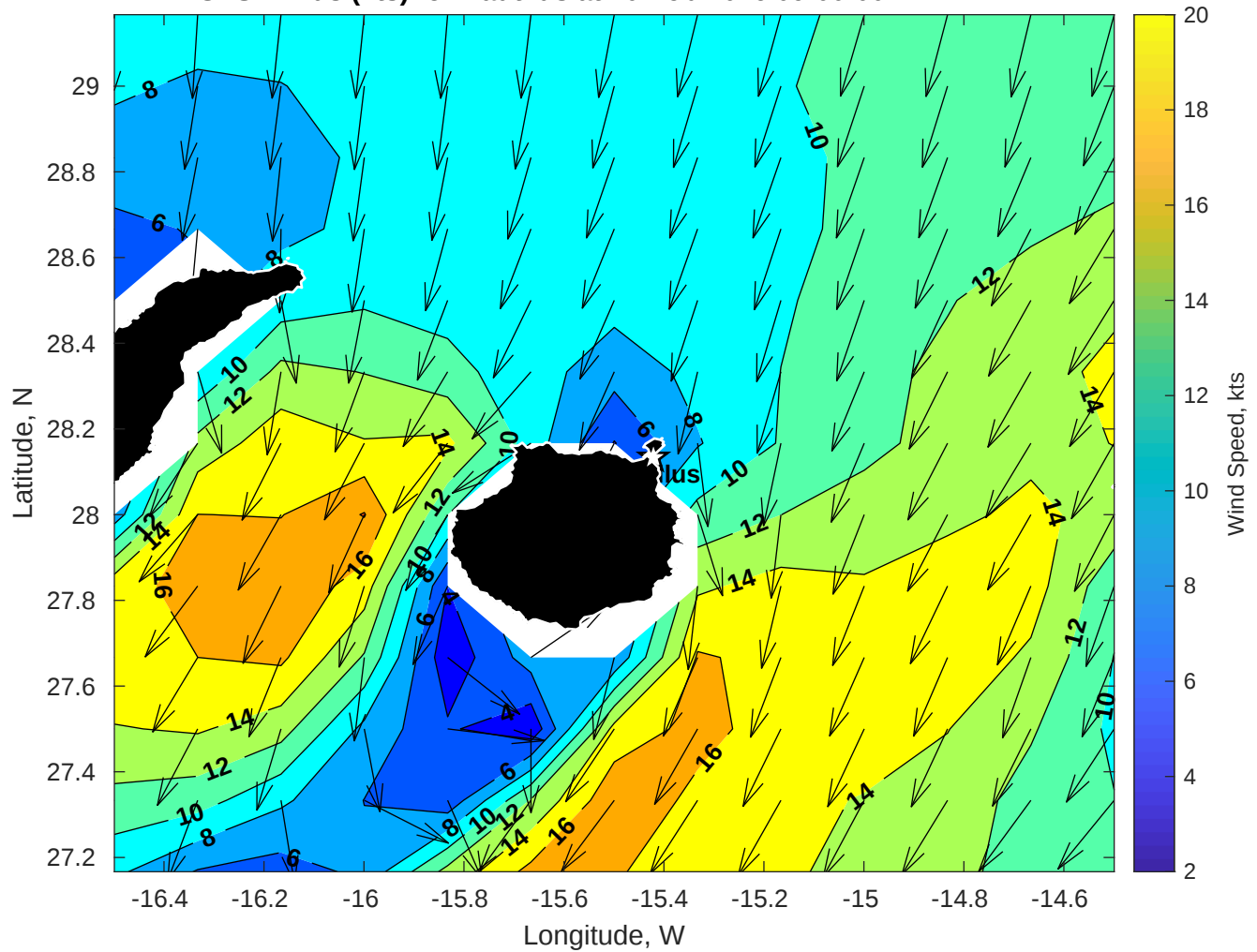
GFS Winds (kts) for Nautilus at 10-Feb-2026 09:00:00
