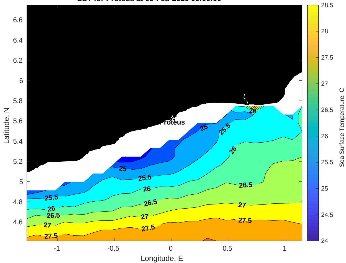
SST for Proteus at 09-Feb-2026 00:00:00
