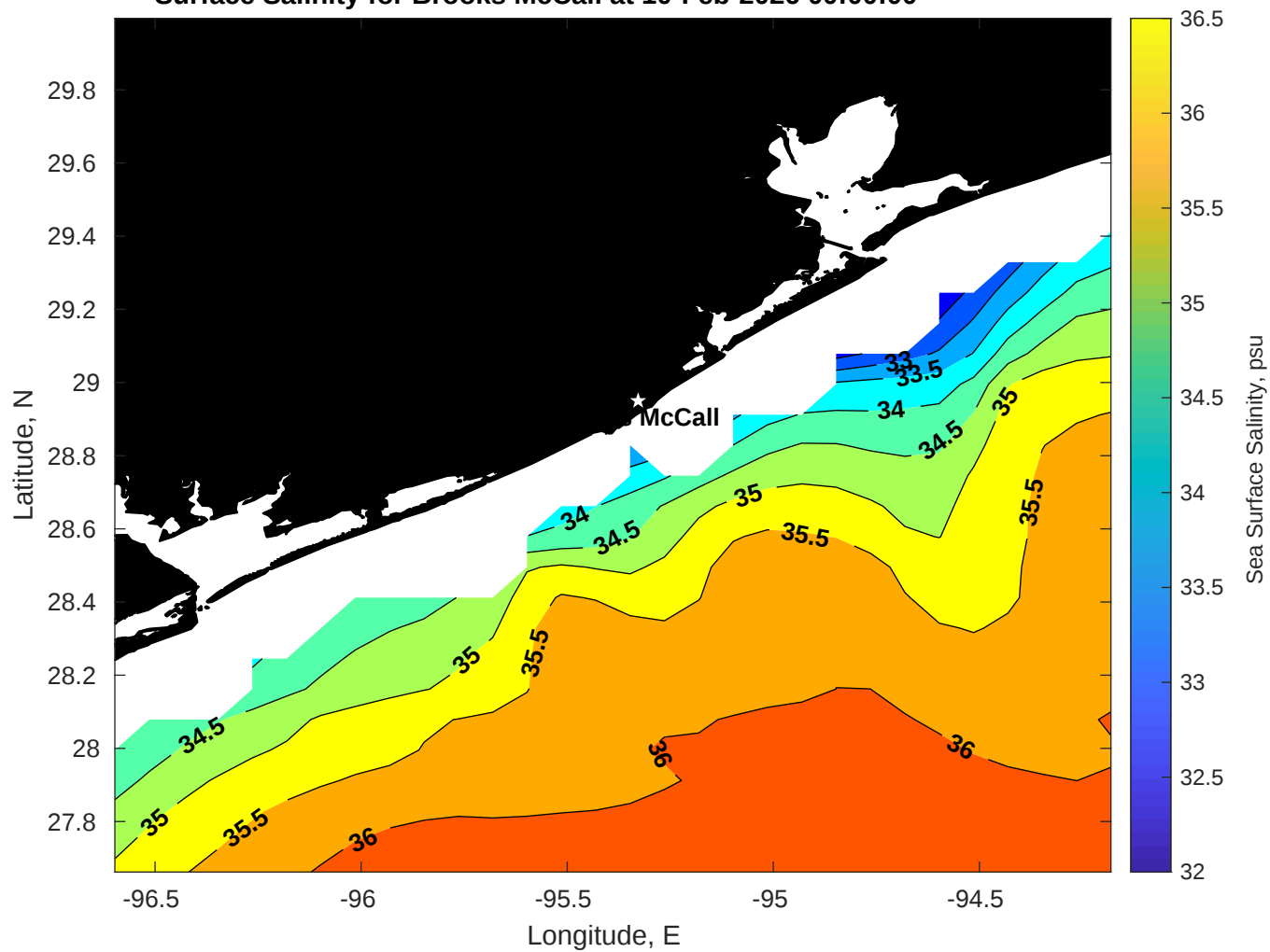
Surface Salinity for Brooks McCall at 10-Feb-2026 00:00:00
