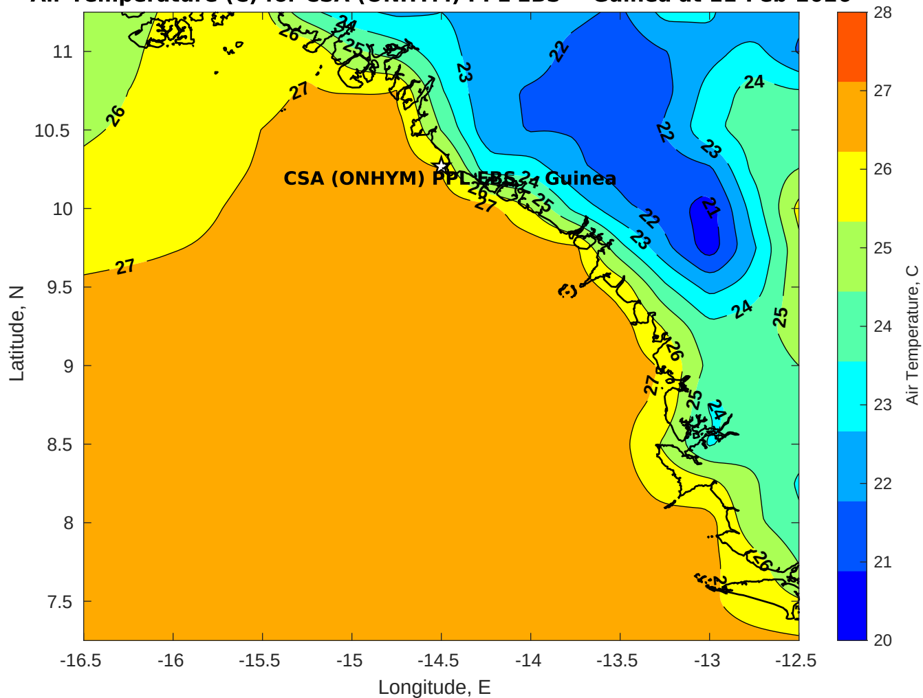
Air Temperature (C) for CSA (ONHYM) PPL EBS - Guinea at 11-Feb-2026
