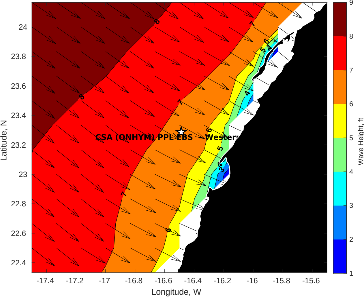
GFS Wave Height (ft) for CSA (ONHYM) PPL EBS - Western Sahara at 11-Feb-2026 09:00:00
