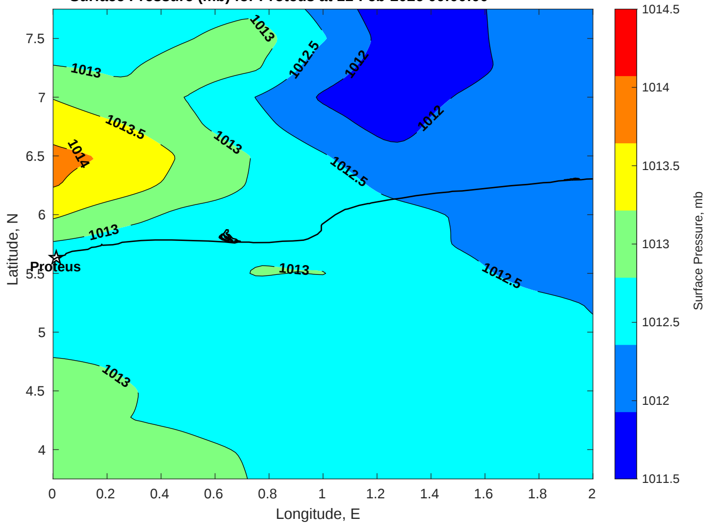
Surface Pressure (mb) for Proteus at 11-Feb-2026 00:00:00
