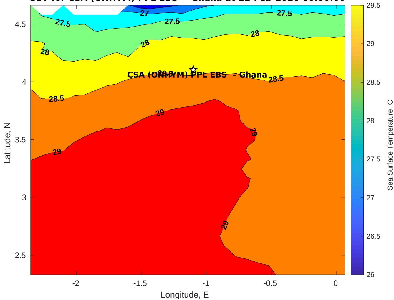
SST for CSA (ONHYM) PPL EBS - Ghana at 11-Feb-2026 00:00:00
