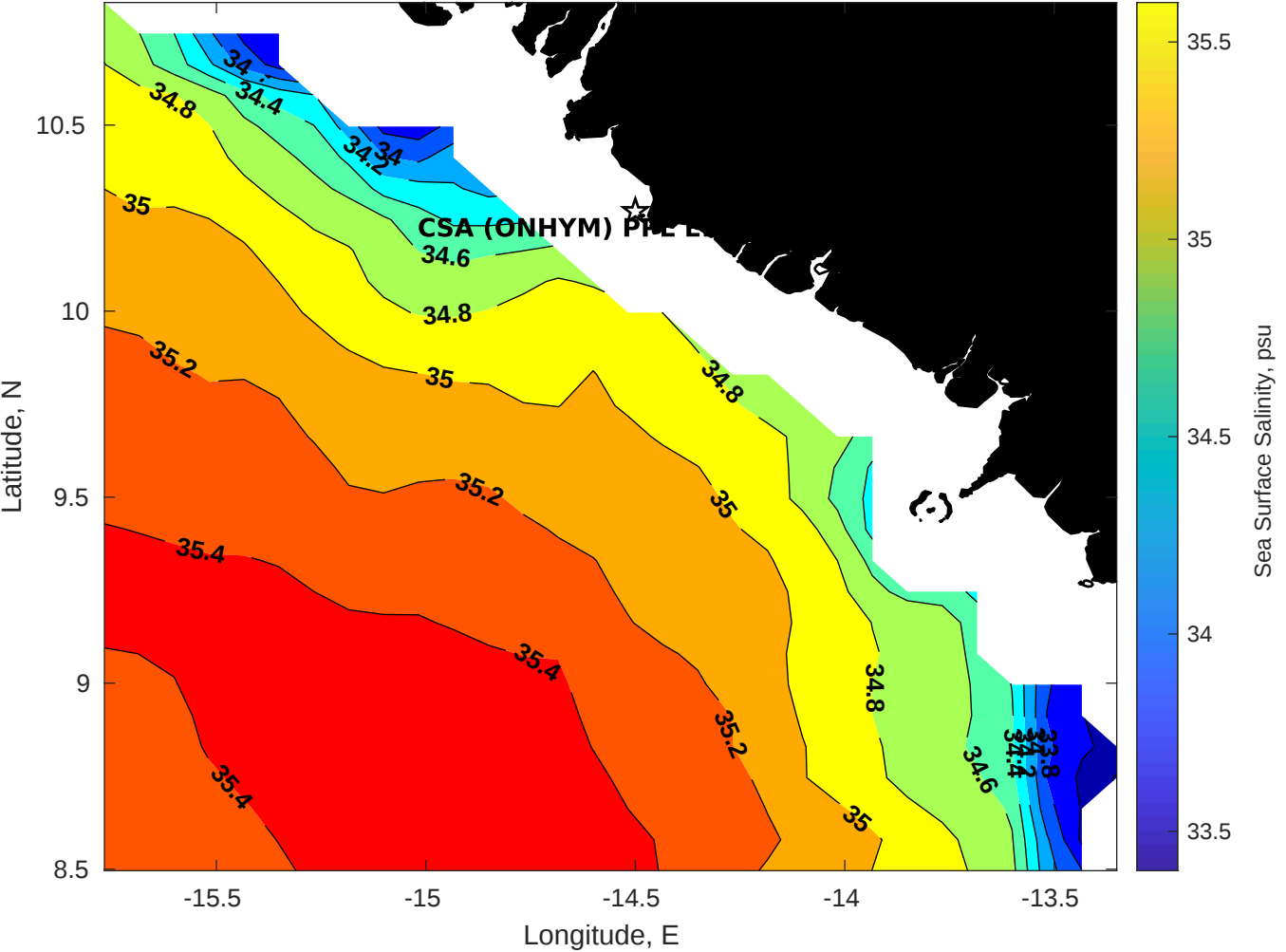
Surface Salinity for CSA (ONHYM) PPL EBS - Guinea at 11-Feb-2026 00:00:00
