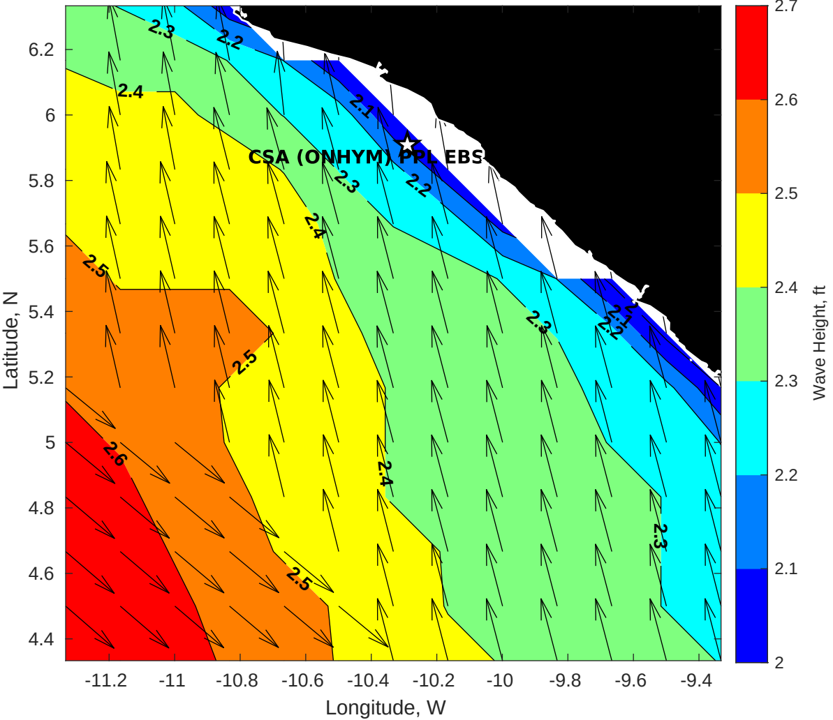
GFS Wave Height (ft) for CSA (ONHYM) PPL EBS - Liberia at 12-Feb-2026 09:00:00
