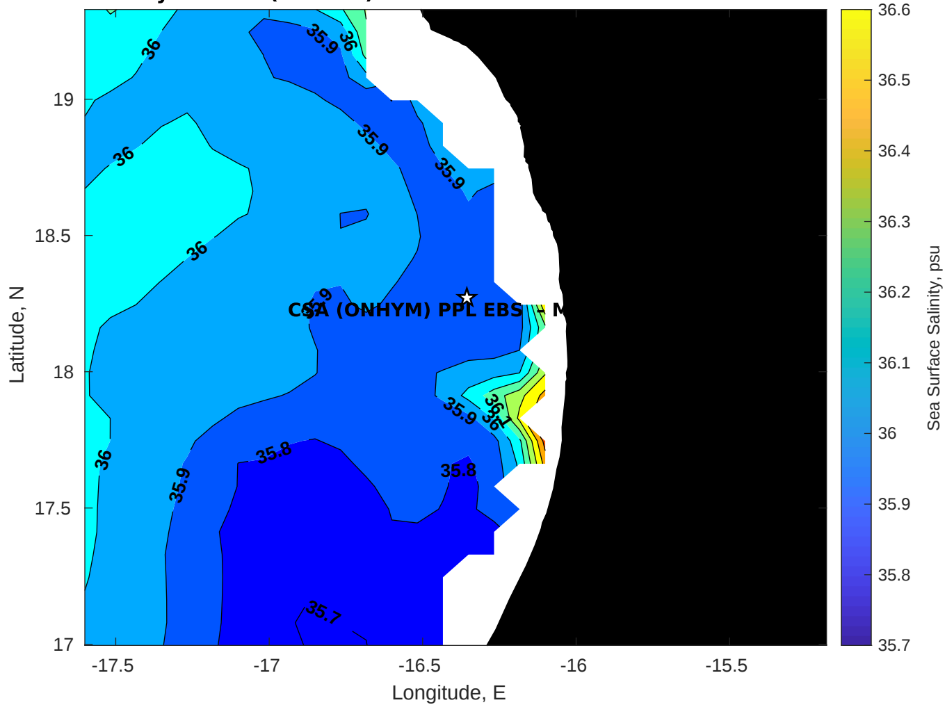
Surface Salinity for CSA (ONHYM) PPL EBS - Mauritania at 11-Feb-2026 00:00:00
