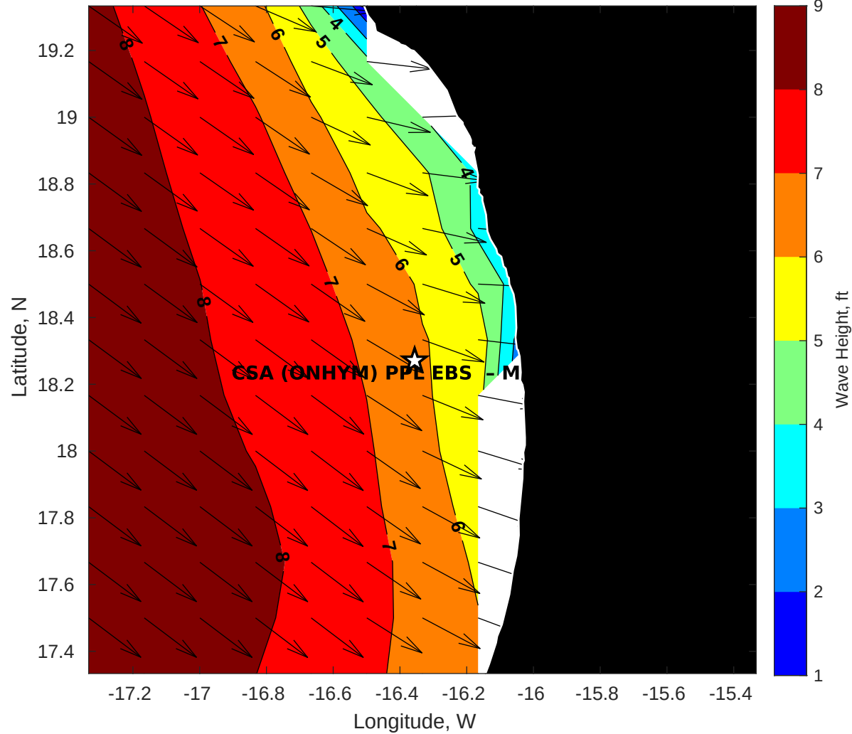
GFS Wave Height (ft) for CSA (ONHYM) PPL EBS - Mauritania at 12-Feb-2026 09:00:00
