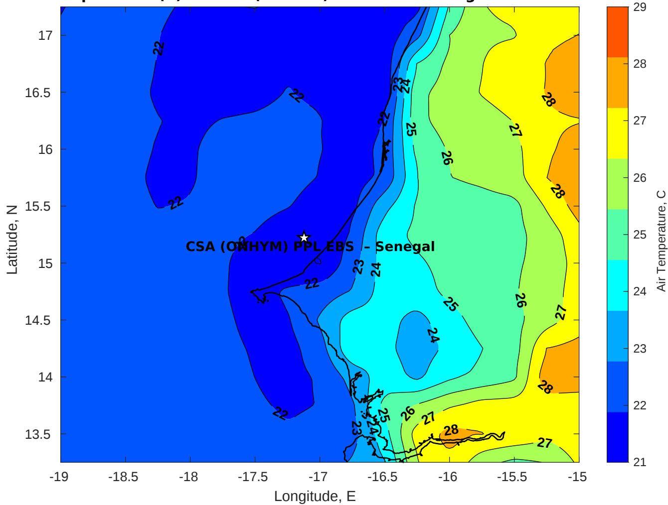
Air Temperature (C) for CSA (ONHYM) PPL EBS - Senegal at 12-Feb-2026
