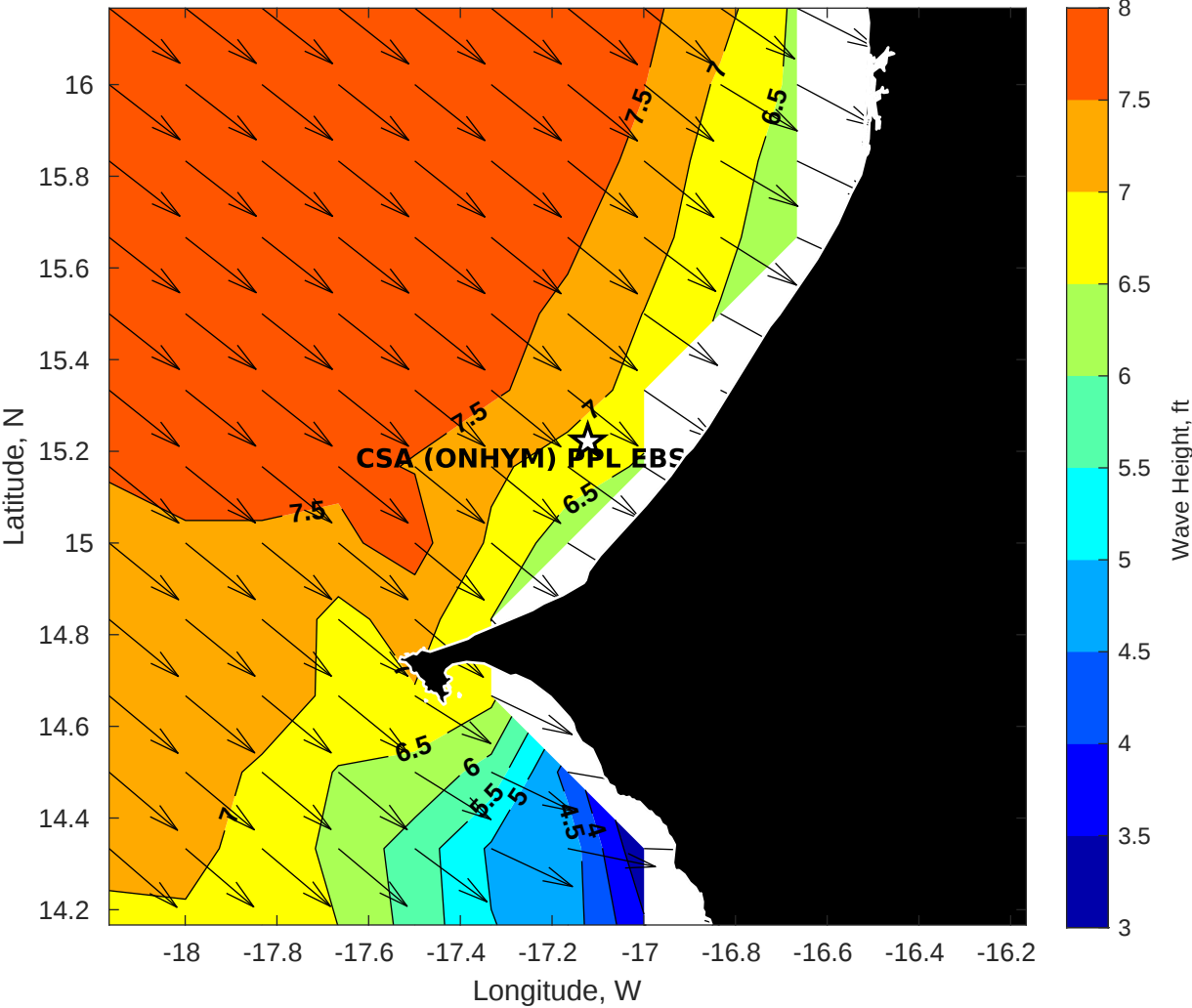
GFS Wave Height (ft) for CSA (ONHYM) PPL EBS - Senegal at 12-Feb-2026 09:00:00
