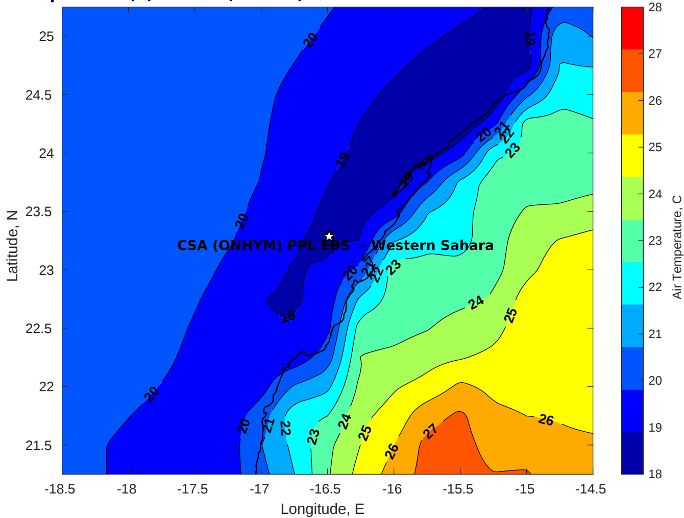
Air Temperature (C) for CSA (ONHYM) PPL EBS - Western Sahara at 12-Feb-2026
