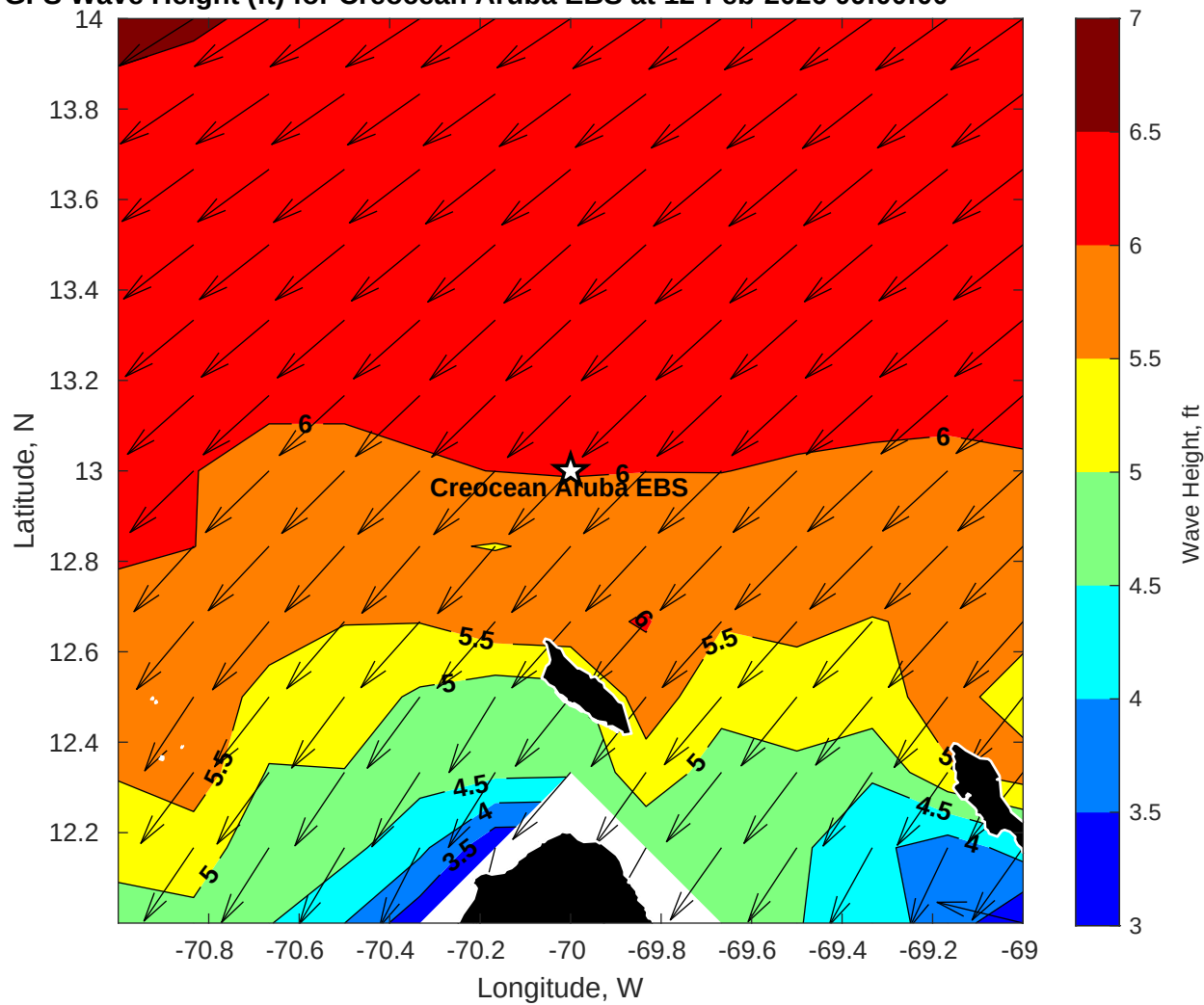
GFS Wave Height (ft) for Creoccean Aruba EBS at 12-Feb-2026 09:00:00
