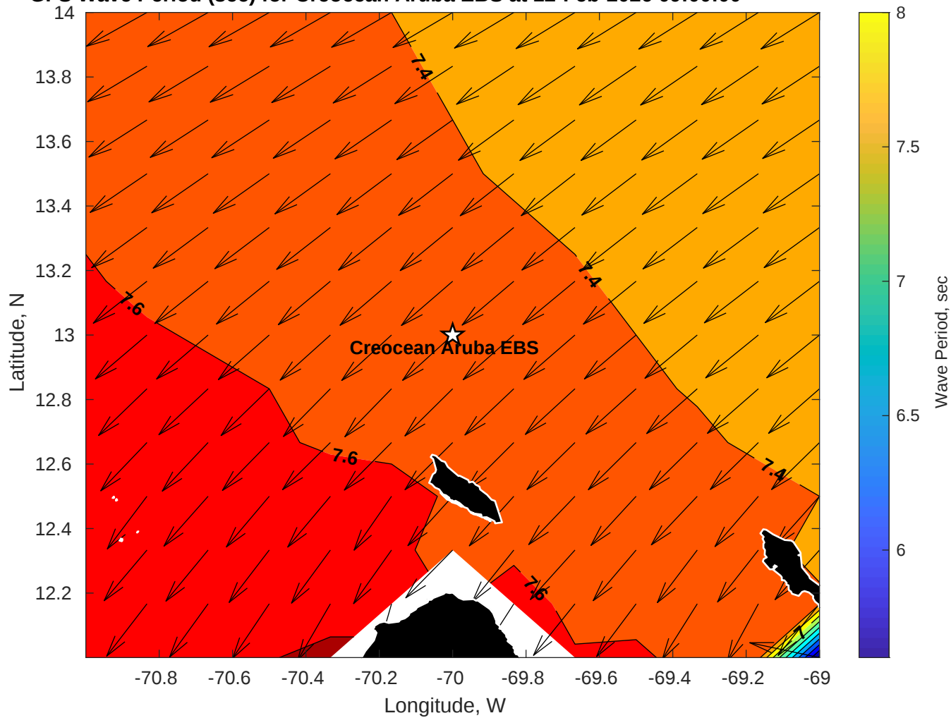
GFS Wave Period (sec) for Creoecean Aruba EBS at 12-Feb-2026 09:00:00
