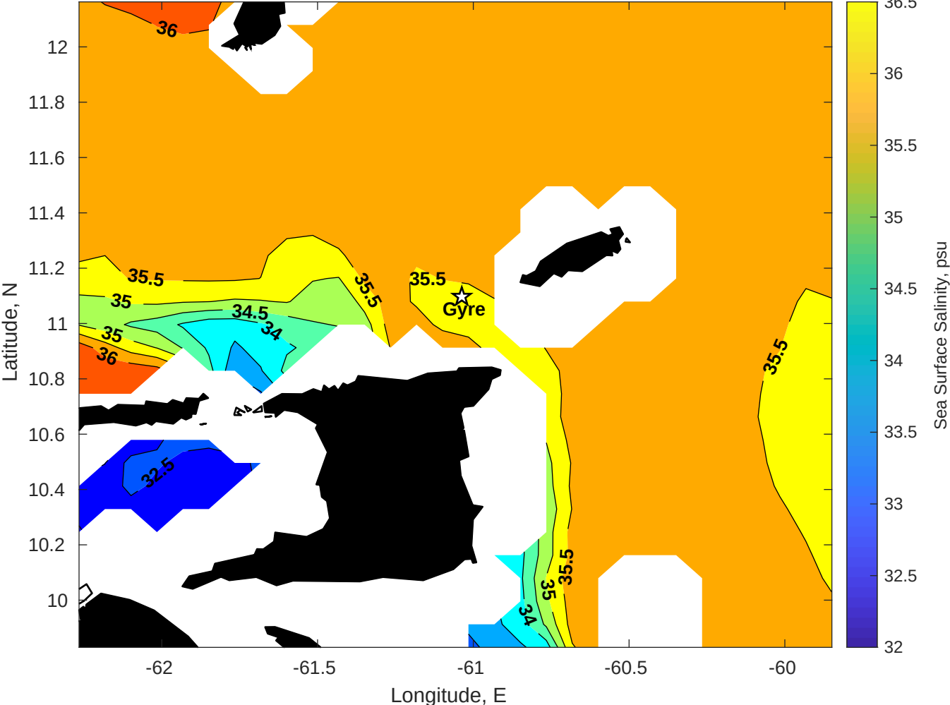
Surface Salinity for Gyre at 11-Feb-2026 00:00:00
